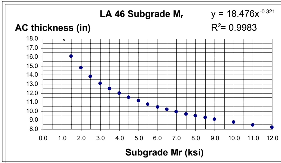
Figure 7 AC versus subgrade M_r (LA 46)
